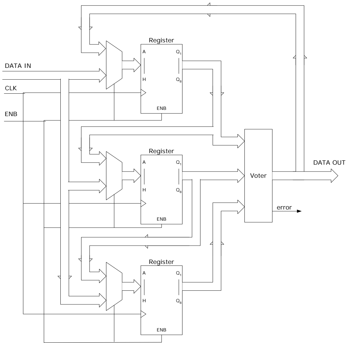
Figure 0-1 Triple Module Redundancy for the Kchip Configuration Registers.
