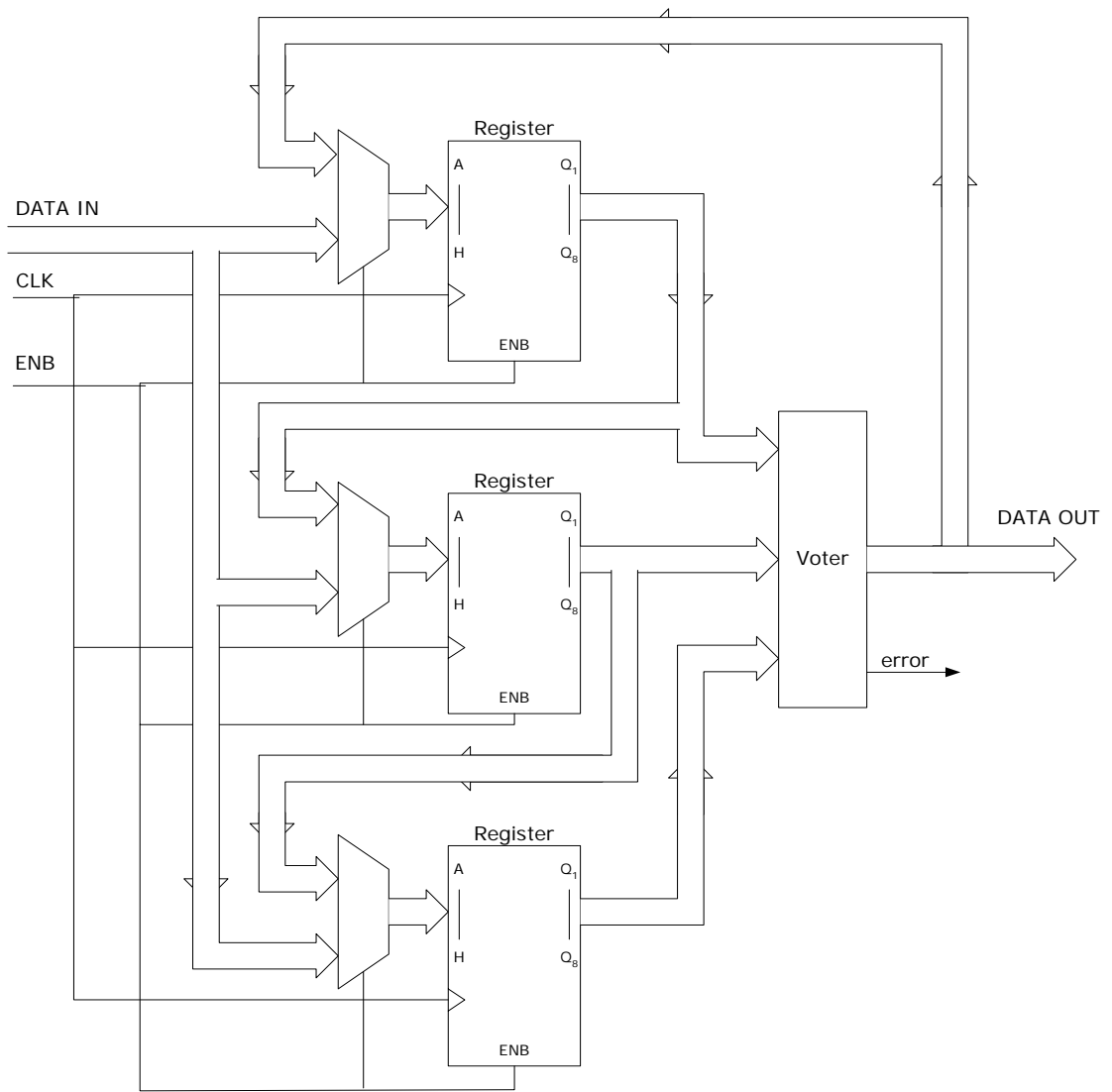
Figure 3-1 Triple Module Redundancy for the Kchip Configuration Registers.
