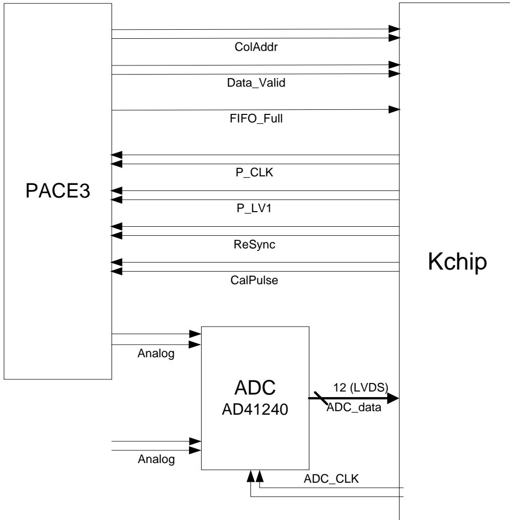
Figure 2-2 PACE3 to Kchip interface.
