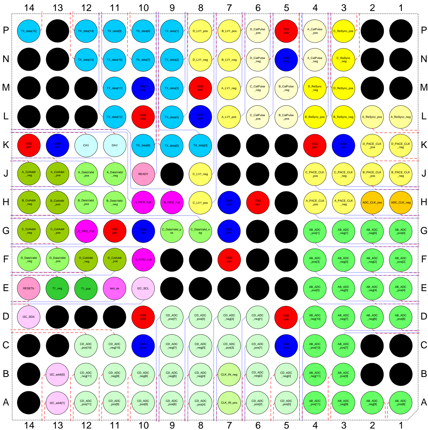
FPBGA-196 TOP VIEW (routing)
